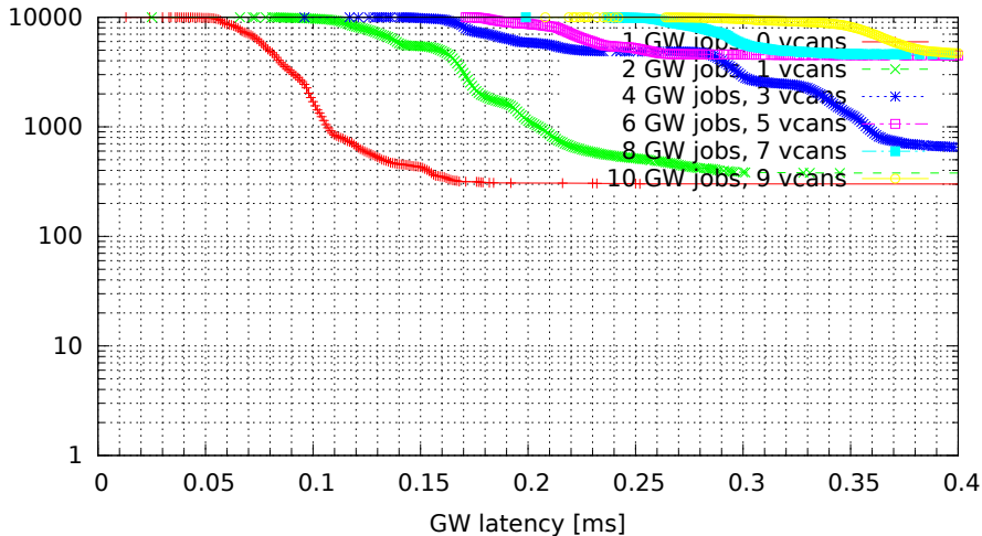
Chained GWs on multiple VCAN interfaces (GW kernel 3.0.4-00007-g1c8c373, Traffic onetotime, Load eth)
