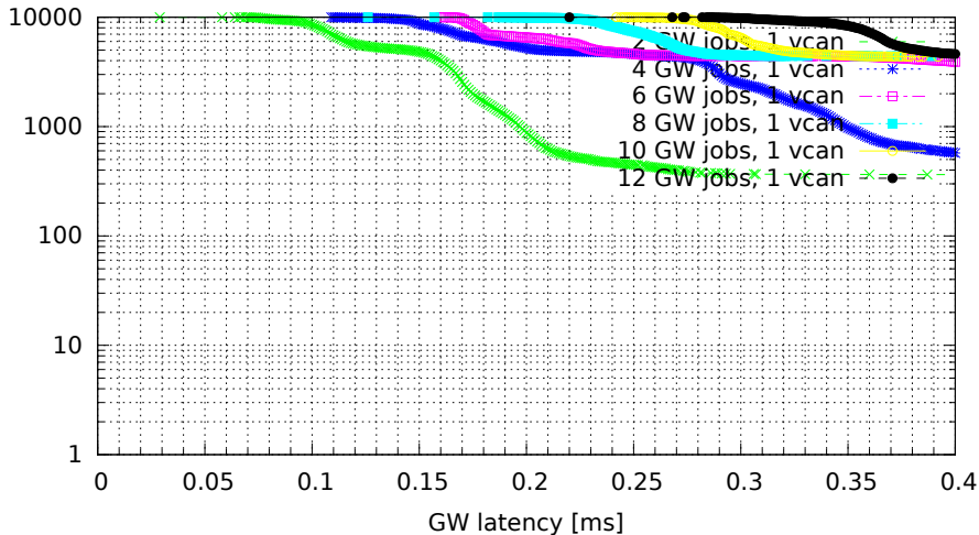
Chained GWs on a single VCAN interface (GW kernel 3.0.4-00007-g1c8c373, Traffic onetatime, Load eth)
