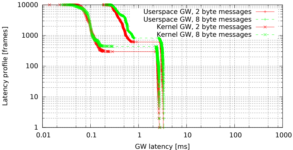
Kernel vs. userspace GW, no modifications (GW kernel 3.0.4-00007-g1c8c373, Traffic oneatatime, Load eth)
