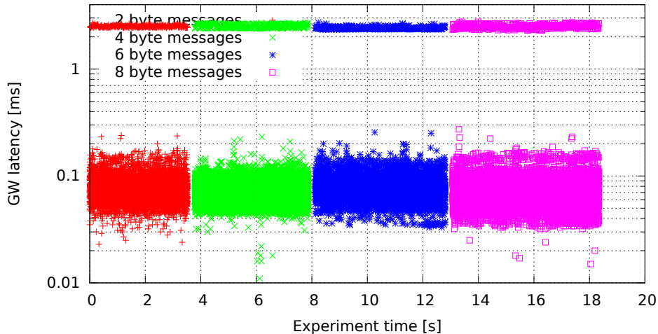
Single GW rule for all messages, no modifications (GW kernel 3.0.4-00007-g1c8c373, Traffic onetatime, Load eth)
