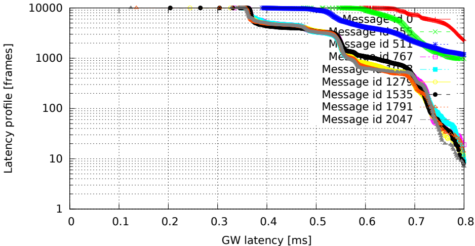
2048 GW rules (one per id, mask 0x7FF), no modifications (GW kernel 3.0.4-00007-g1c8c373, Traffic onetotime, Load eth)
