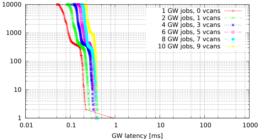
Chained GWs on multiple VCAN interfaces (GW kernel 3.0.4-00007-g1c8c373, Traffic oneatatime, Load cpu)
