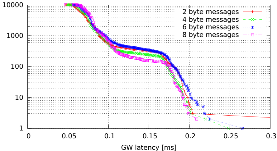
Single GW rule for all messages, no modifications (GW kernel 3.0.4-00007-g1c8c373, Traffic oneatatime, Load cpu)
