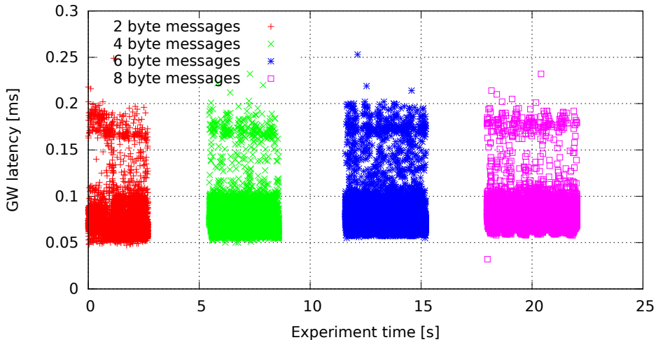
Single GW rule for all messages, no modifications, high (soft)irq task priority (GW kernel 3.0.4-00007-g1c8c373, Traffic oneatatime, Load cpu)
