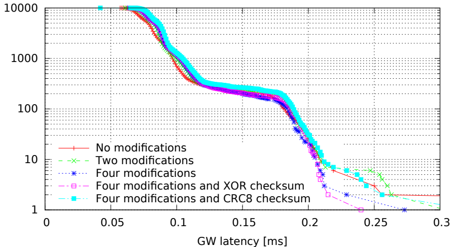
Single GW rule for all messages with modifications, 8 byte messages (GW kernel 3.0.4-00007-g1c8c373, Traffic oneatatime, Load cpu)
