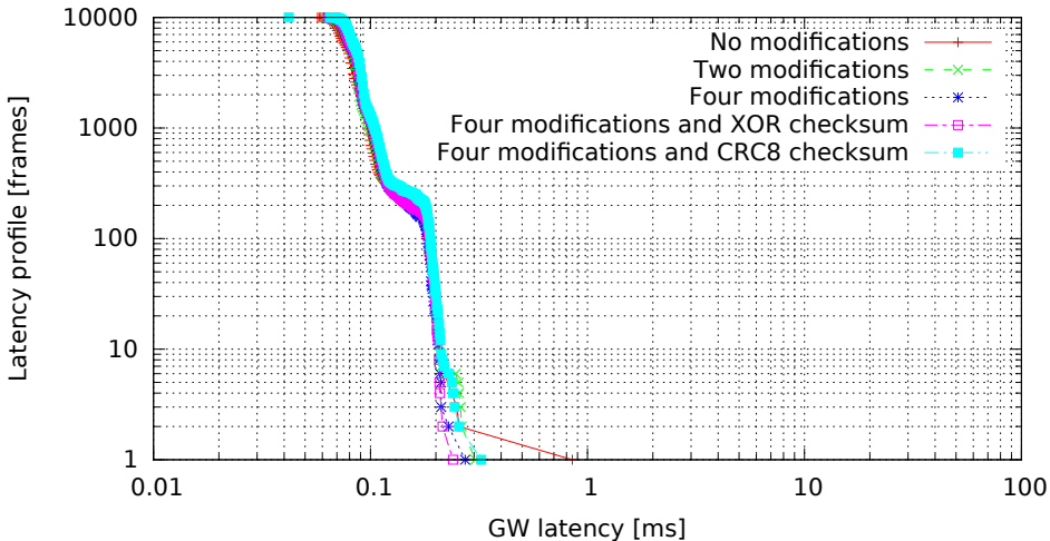
Single GW rule for all messages with modifications, 8 byte messages (GW kernel 3.0.4-00007-g1c8c373, Traffic oneatatime, Load cpu)
