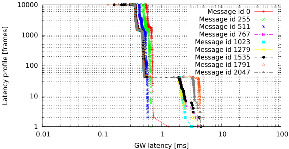
2048 GW rules (one per id, mask 0x7FF), no modifications (GW kernel 3.0.4-00007-g1c8c373, Traffic onetatime, Load cpu)
