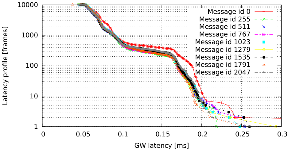
2048 GW rules (one per id, mask C00007FF), no modifications (GW kernel 3.0.4-00007-g1c8c373, Traffic oneatatime, Load cpu)
