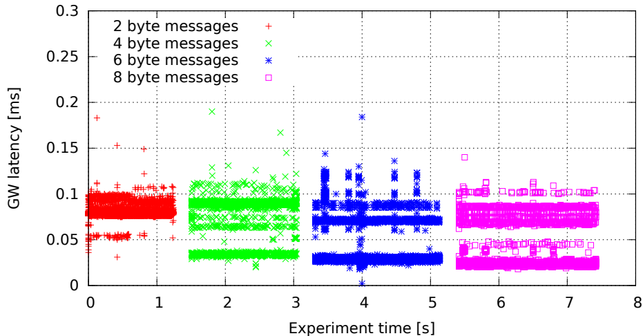
Single GW rule for all messages, no modifications (GW kernel 3.0.4-00007-g1c8c373, Traffic flood, Load none)
