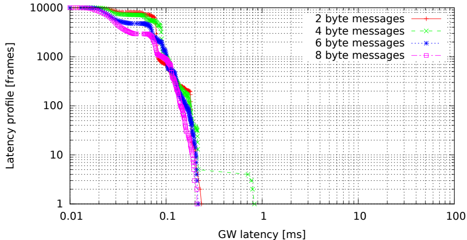
Single GW rule for all messages, no modifications (GW kernel 3.0.4-00007-g1c8c373, Traffic flood, Load cpu)
