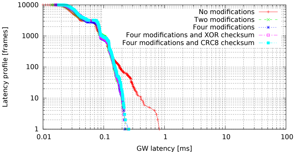
Single GW rule for all messages with modifications, 8 byte messages (GW kernel 3.0.4-00007-g1c8c373, Traffic flood, Load cpu)
