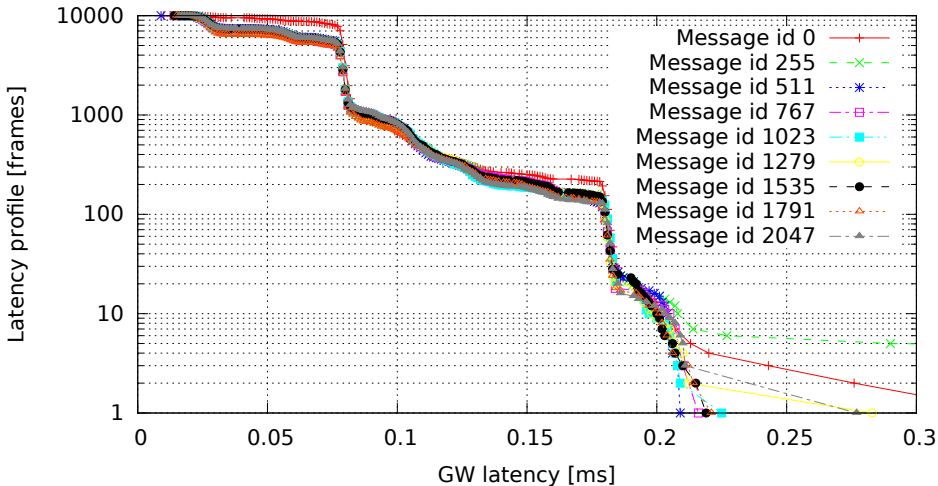
2048 GW rules (one per id, mask C00007FF), no modifications (GW kernel 3.0.4-00007-g1c8c373, Traffic flood, Load cpu)
