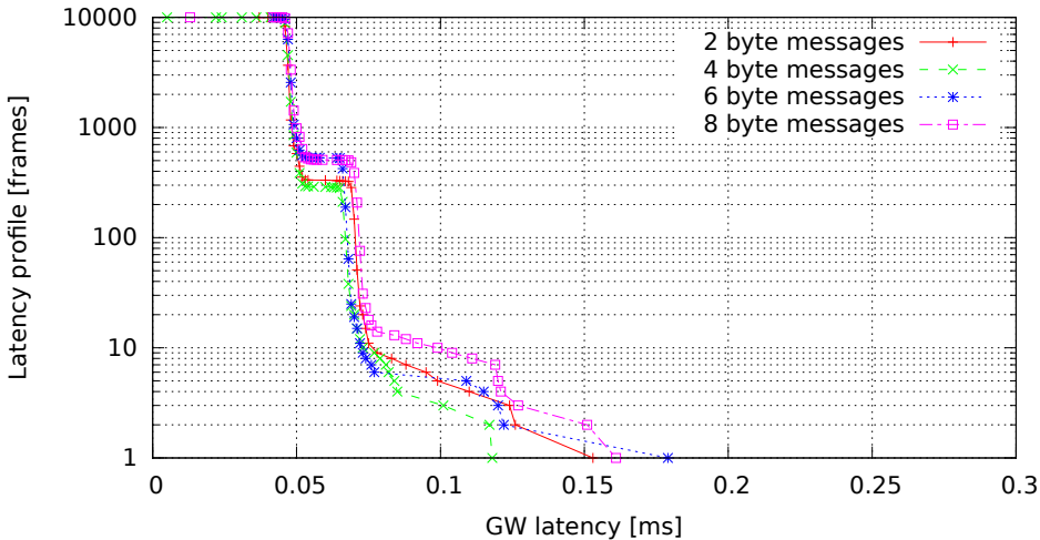
Single GW rule for all messages, no modifications (GW kernel 2.6.36.2-00015-g4f1bc4e, Traffic oneatatime, Load none)
