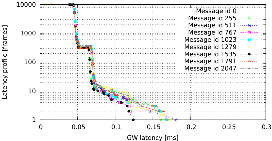
2048 GW rules (one per id, mask C00007FF), no modifications (GW kernel 2.6.36.2-00015-g4f1bc4e, Traffic oneatatime, Load none)
