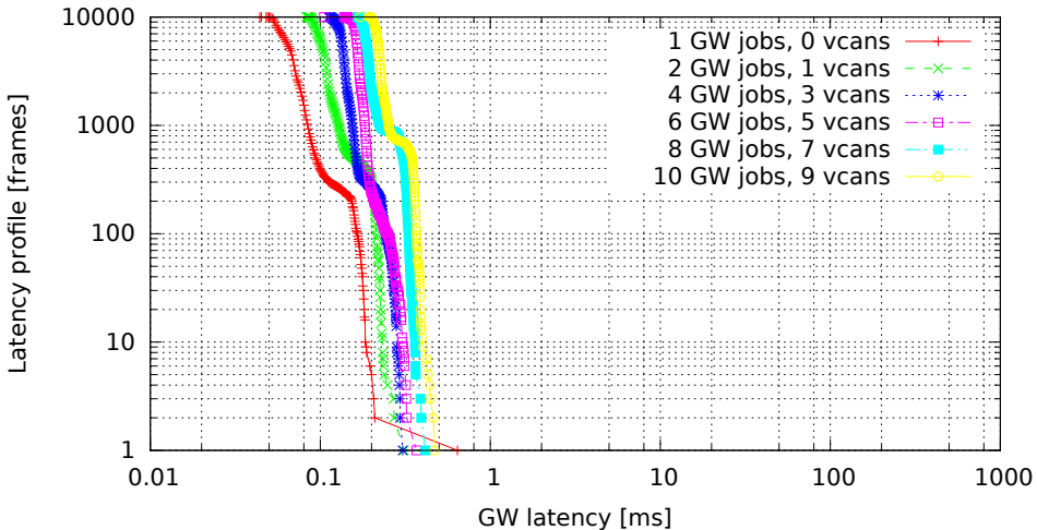
Chained GWs on multiple VCAN interfaces (GW kernel 2.6.36.2-00015-g4f1bc4e, Traffic oneatatime, Load cpu)
