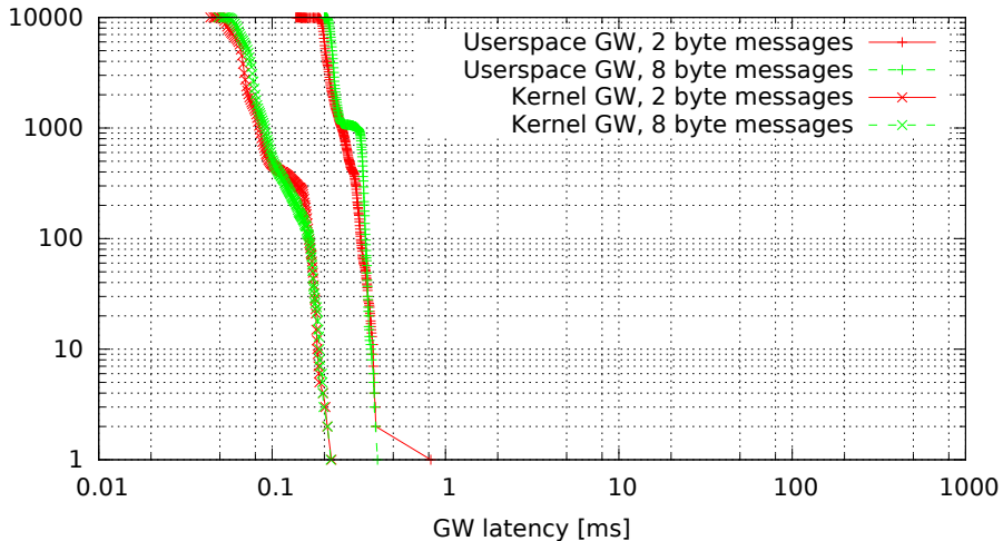
Kernel vs. userspace GW, no modifications (GW kernel 2.6.36.2-00015-g4f1bc4e, Traffic oneatatime, Load cpu)
