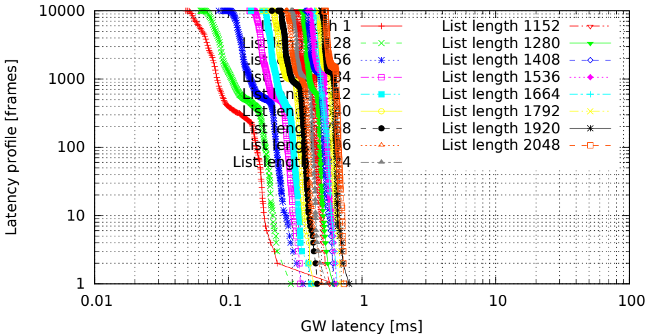
Different lengths of filter list, only the last one matches (GW kernel 2.6.36.2-00015-g4f1bc4e, Traffic oneatatime, Load cpu)
