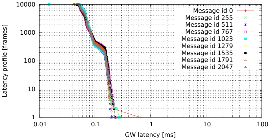
2048 GW rules (one per id, mask C00007FF), no modifications (GW kernel 2.6.36.2-00015-g4f1bc4e, Traffic oneatatime, Load cpu)
