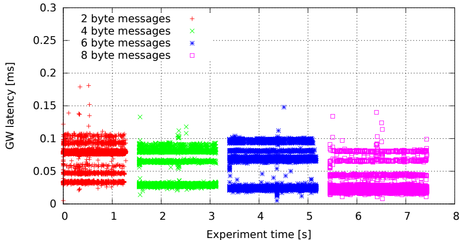
Single GW rule for all messages, no modifications, high (soft)irq task priority (GW kernel 2.6.36.2-00015-g4f1bc4e, Traffic flood, Load none)
