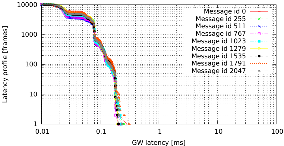
2048 GW rules (one per id, mask C00007FF), no modifications (GW kernel 2.6.36.2-00015-g4f1bc4e, Traffic flood, Load cpu)
