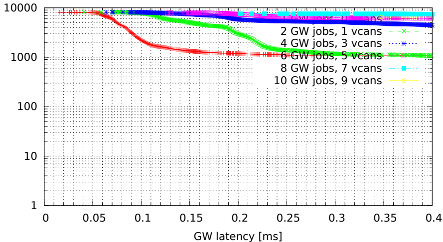
Chained GWs on multiple VCAN interfaces (GW kernel 2.6.36.2-00015-g4f1bc4e, Traffic 50, Load eth)
