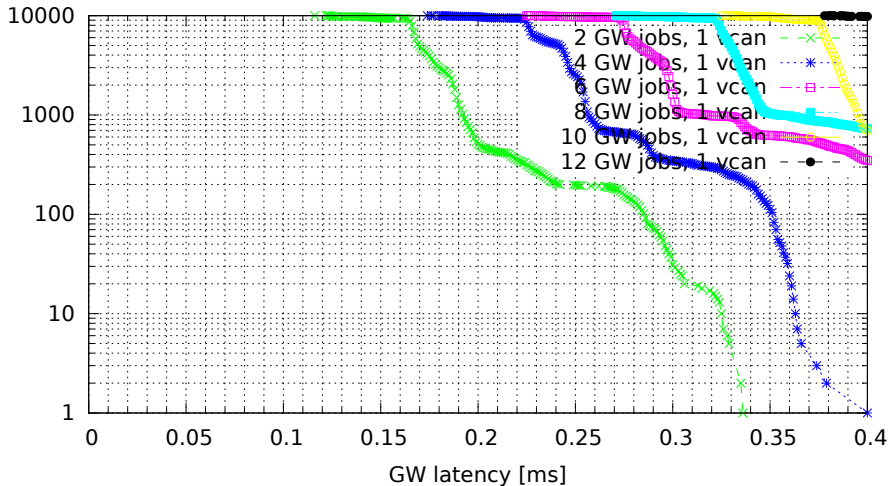
Chained GWs on a single VCAN interface (GW kernel 2.6.33.7-rt29-00004-g92487e4, Traffic oneatatime, Load none)
