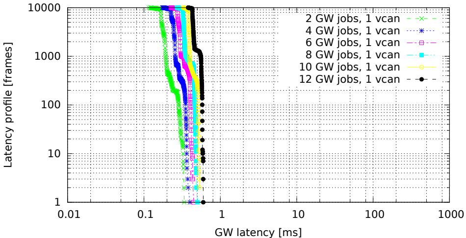
Chained GWs on a single VCAN interface (GW kernel 2.6.33.7-rt29-00004-g92487e4, Traffic oneatatime, Load none)
