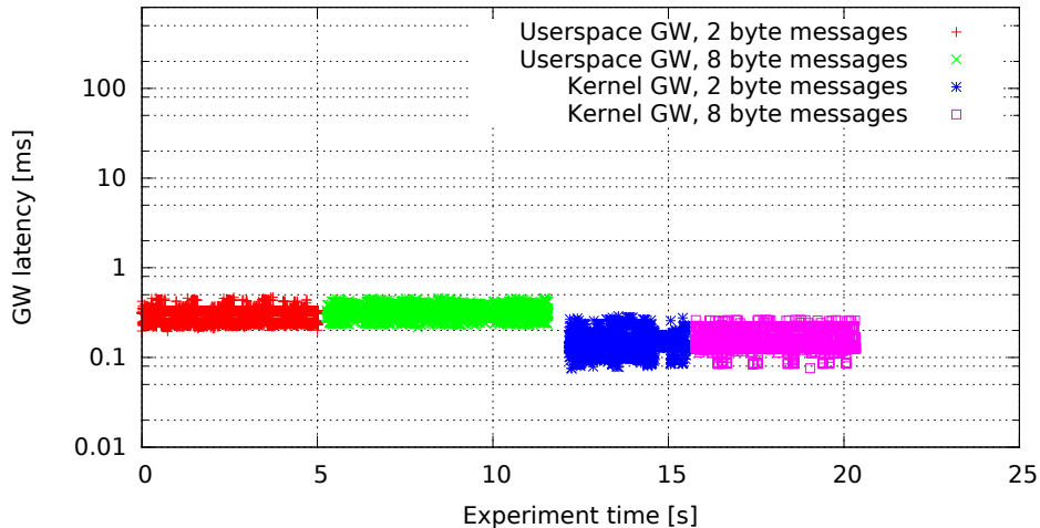
Single GW rule for all messages, no modifications (GW kernel 2.6.33.7-rt29-00004-g92487e4, Traffic oneatatime, Load none)
