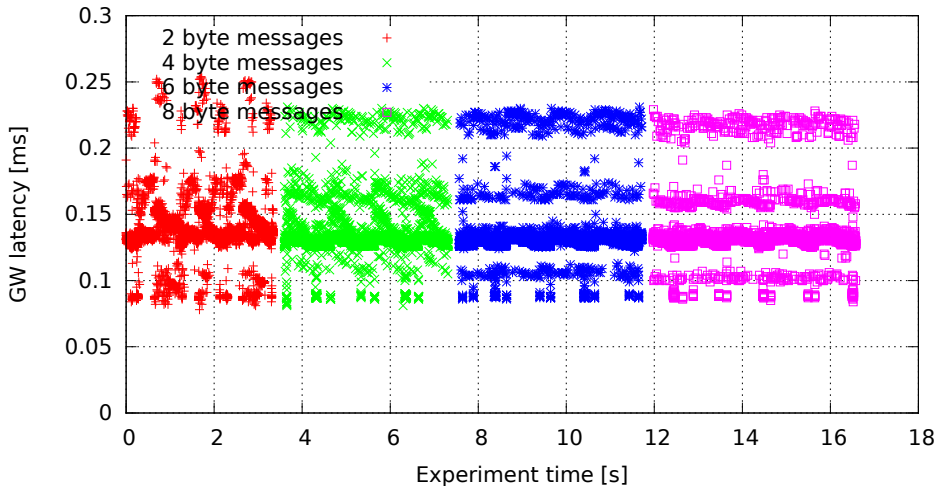
Single GW rule for all messages, no modifications, high (soft)irq task priority (GW kernel 2.6.33.7-rt29-00004-g92487e4, Traffic oneatatime, Load none)
