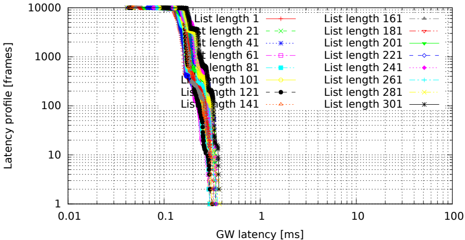
Different lengths of filter list, only the last one matches (GW kernel 2.6.33.7-rt29-00004-g92487e4, Traffic oneatatime, Load none)
