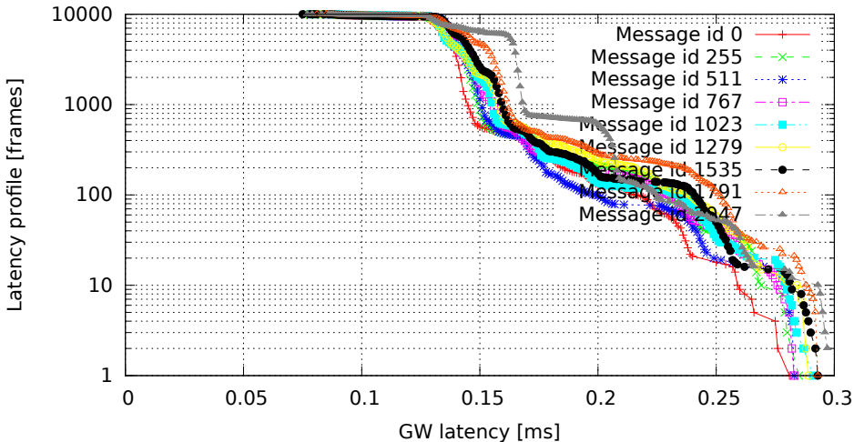
2048 GW rules (one per id, mask C00007FF), no modifications (GW kernel 2.6.33.7-rt29-00004-g92487e4, Traffic oneatatime, Load none)
