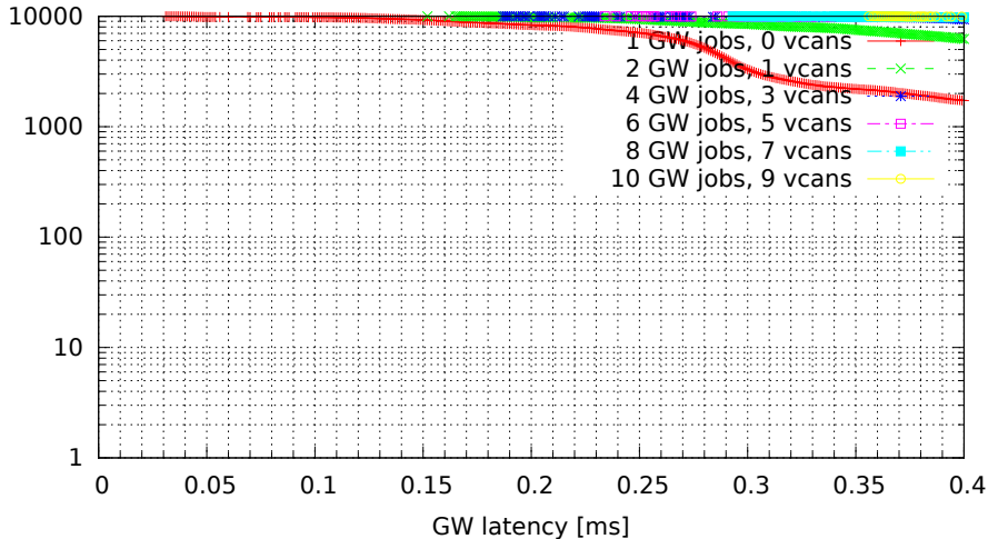
Chained GWs on multiple VCAN interfaces (GW kernel 2.6.33.7-rt29-00004-g92487e4, Traffic onetatime, Load eth)
