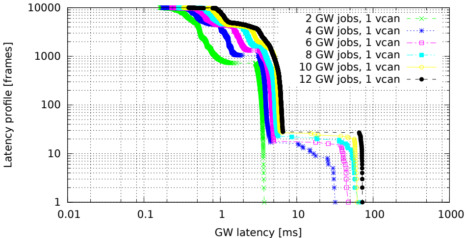
Chained GWs on a single VCAN interface (GW kernel 2.6.33.7-rt29-00004-g92487e4, Traffic onetotime, Load eth)
