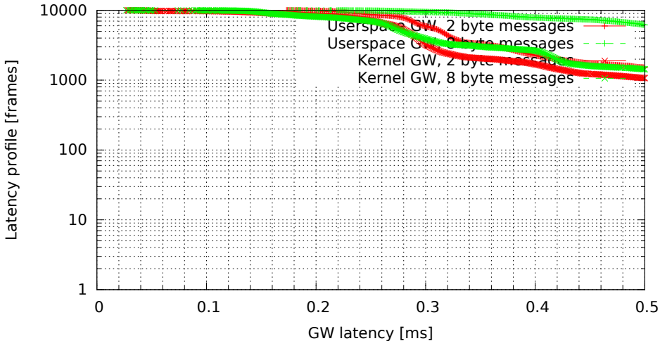
Kernel vs. userspace GW, no modifications (GW kernel 2.6.33.7-rt29-00004-g92487e4, Traffic oneatatime, Load eth)
