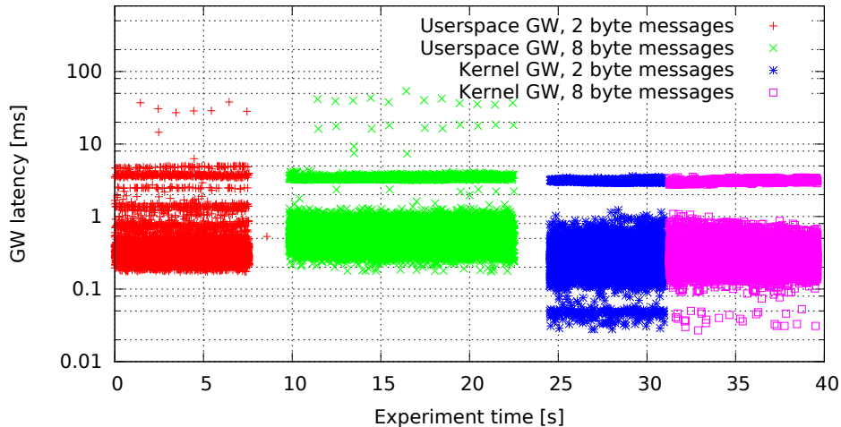
Single GW rule for all messages, no modifications (GW kernel 2.6.33.7-rt29-00004-g92487e4, Traffic oneatatime, Load eth)
