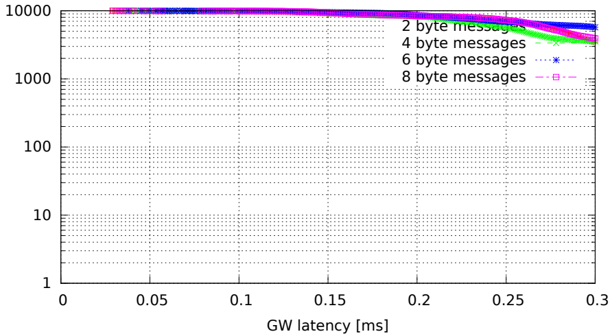
Single GW rule for all messages, no modifications (GW kernel 2.6.33.7-rt29-00004-g92487e4, Traffic onetatime, Load eth)
