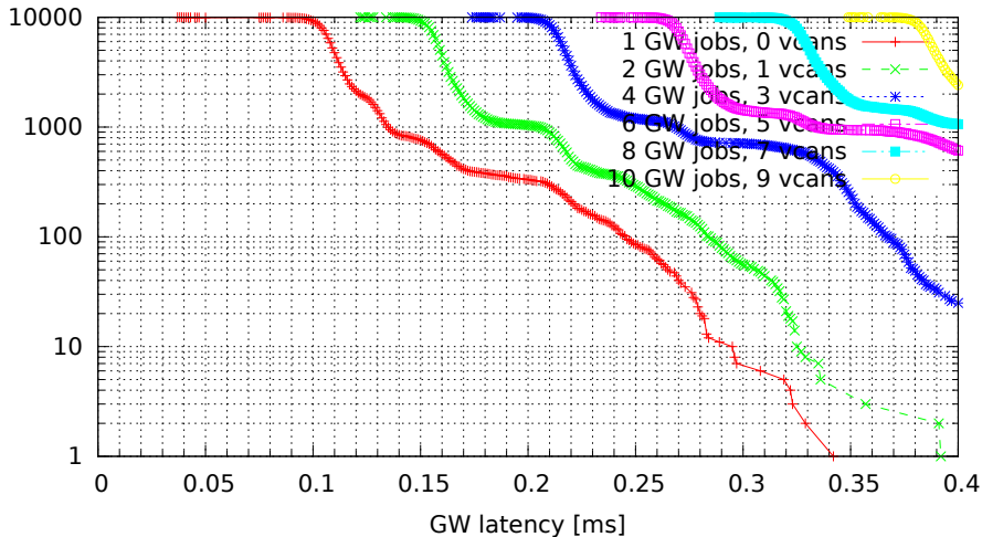
Chained GWs on multiple VCAN interfaces (GW kernel 2.6.33.7-rt29-00004-g92487e4, Traffic oneatatime, Load cpu)
