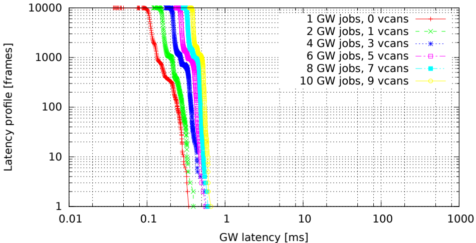
Chained GWs on multiple VCAN interfaces (GW kernel 2.6.33.7-rt29-00004-g92487e4, Traffic oneatatime, Load cpu)
