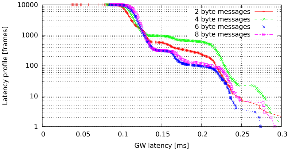
Single GW rule for all messages, no modifications, high (soft)irq task priority (GW kernel 2.6.33.7-rt29-00004-g92487e4, Traffic onetatime, Load cpu)
