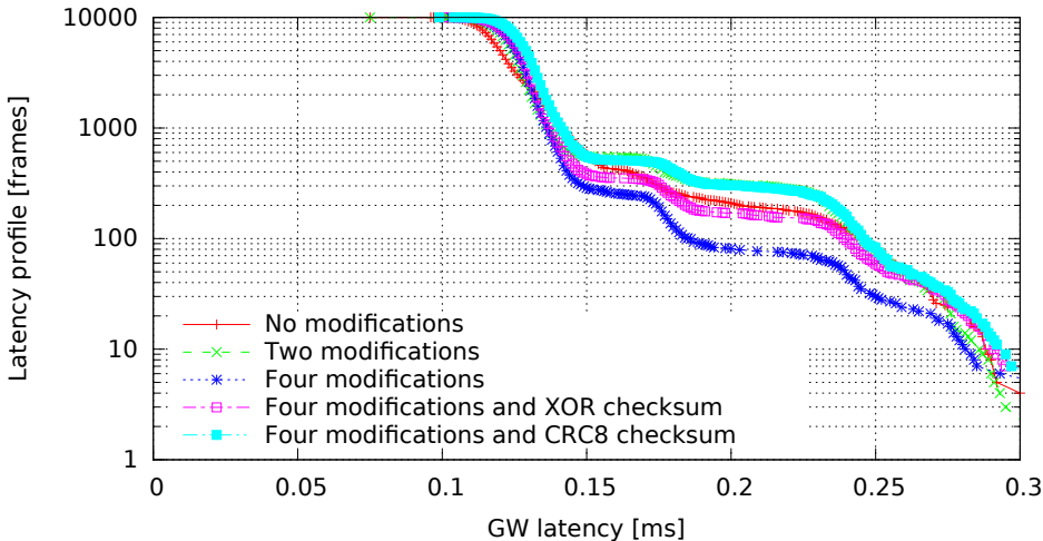
Single GW rule for all messages with modifications, 8 byte messages (GW kernel 2.6.33.7-rt29-00004-g92487e4, Traffic onetatime, Load cpu)
