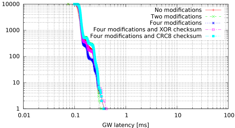
Single GW rule for all messages with modifications, 8 byte messages (GW kernel 2.6.33.7-rt29-00004-g92487e4, Traffic oneatatime, Load cpu)
