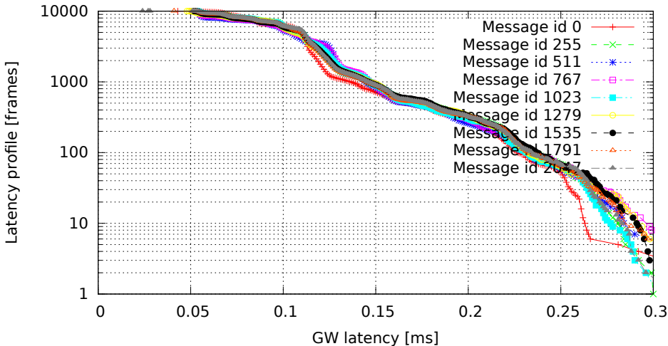
2048 GW rules (one per id, mask C00007FF), no modifications (GW kernel 2.6.33.7-rt29-00004-g92487e4, Traffic flood, Load cpu)
