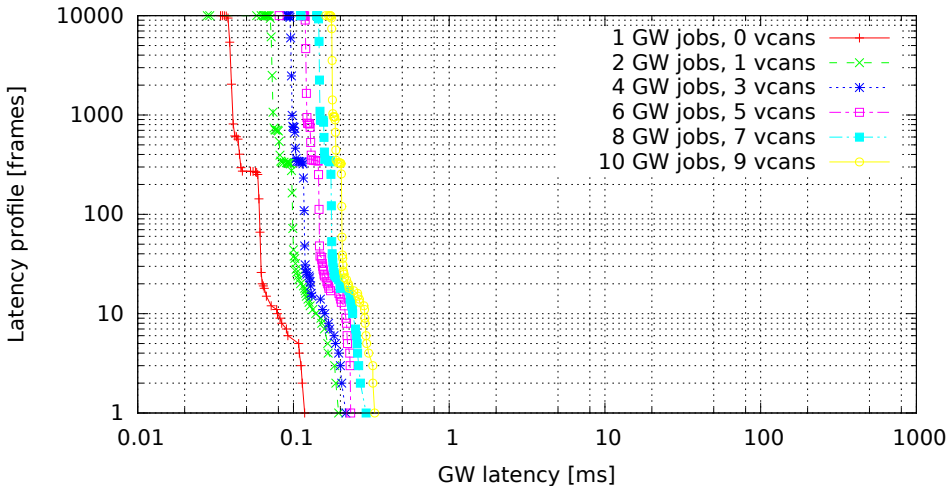
Chained GWs on multiple VCAN interfaces (GW kernel 2.6.33.7-00007-g9c0ff90, Traffic oneatatime, Load none)
