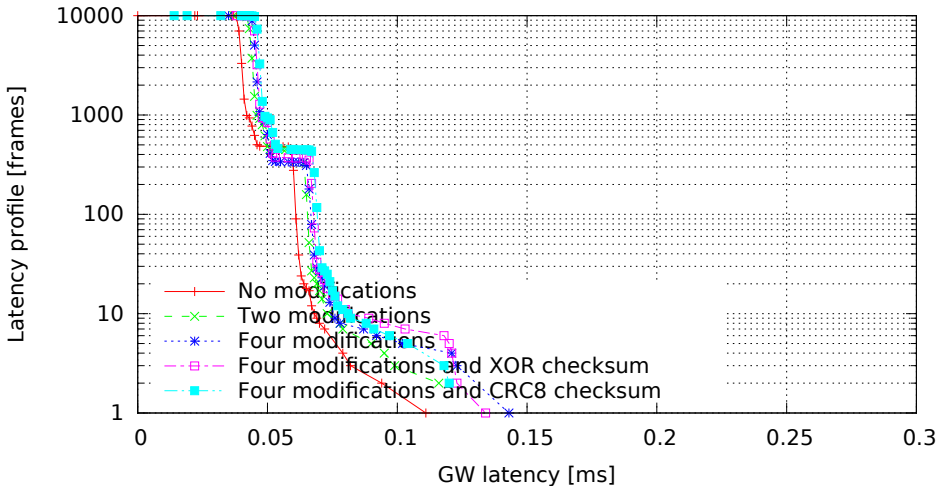
Single GW rule for all messages with modifications, 8 byte messages (GW kernel 2.6.33.7-00007-g9c0ff90, Traffic onetotime, Load none)
