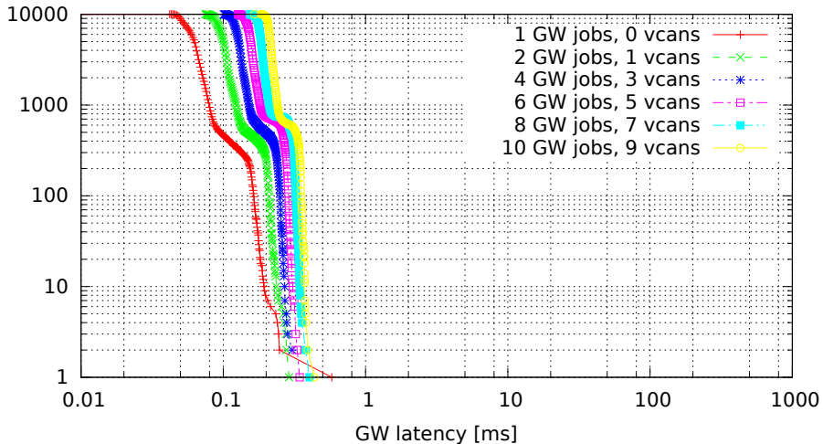
Chained GWs on multiple VCAN interfaces (GW kernel 2.6.33.7-00007-g9c0ff90, Traffic oneatatime, Load cpu)
