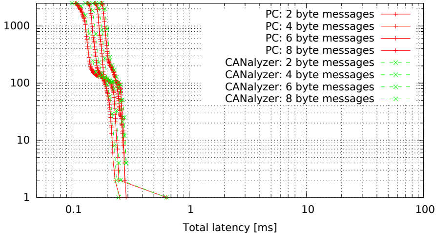
Measurement precision: PC versus CANalyzer (GW kernel 2.6.33.7-00007-g9c0ff90, Traffic oneatatime, Load cpu)
