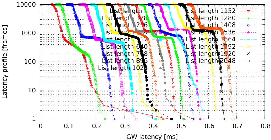
Different lengths of filter list, only the last one matches (GW kernel 2.6.33.7-00007-g9c0ff90, Traffic oneatatime, Load cpu)
