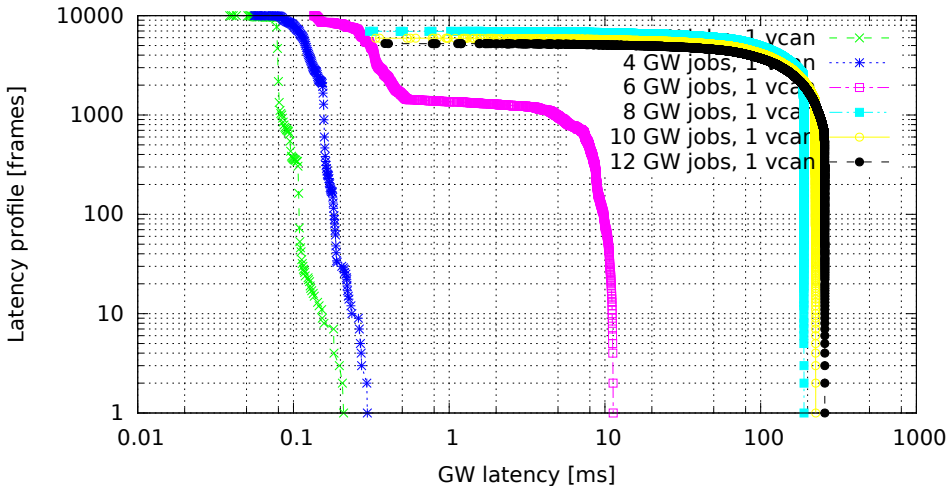
Chained GWs on a single VCAN interface (GW kernel 2.6.33.7-00007-g9c0ff90, Traffic flood, Load none)
