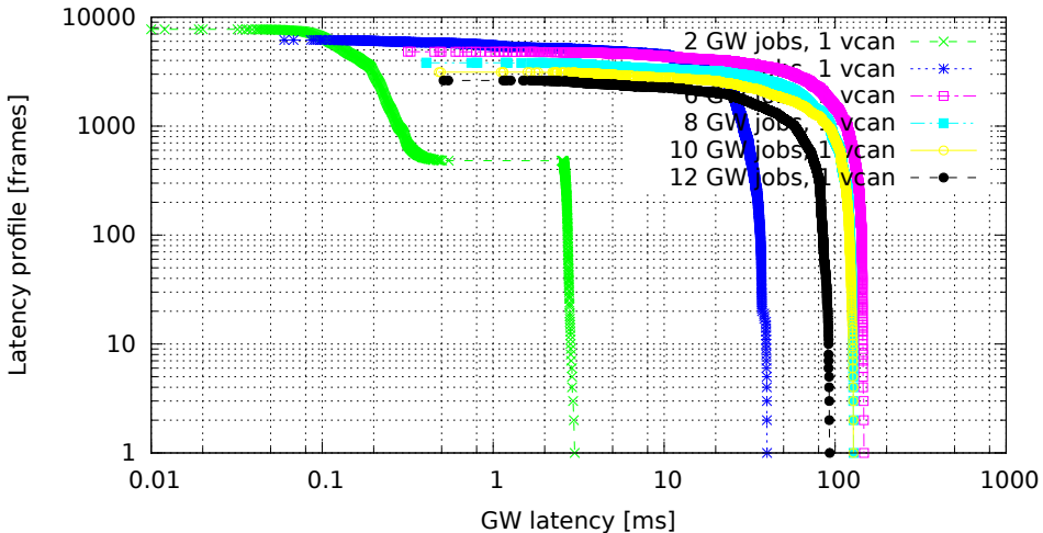
Chained GWs on a single VCAN interface (GW kernel 2.6.33.7-00007-g9c0ff90, Traffic flood, Load eth)
