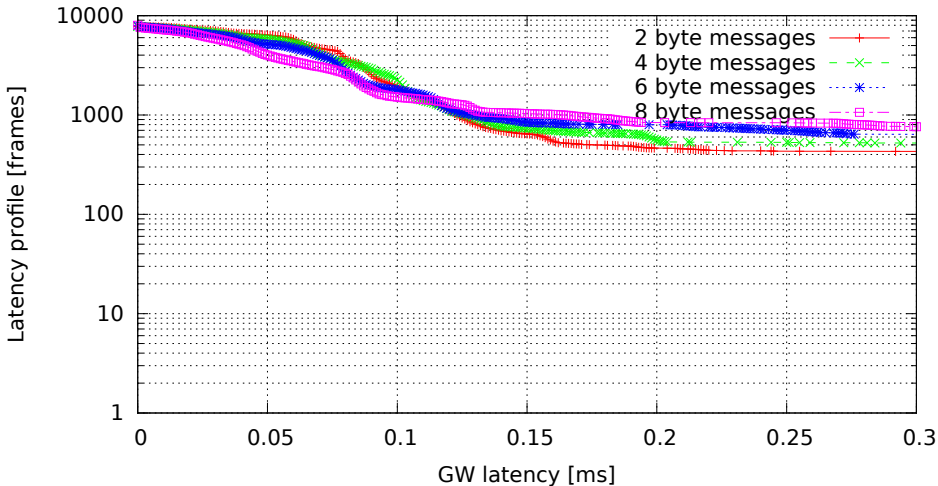
Single GW rule for all messages, no modifications, high (soft)irq task priority (GW kernel 2.6.33.7-00007-g9c0ff90, Traffic flood, Load eth)
